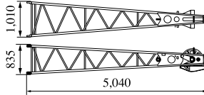
9.1 m Special Insert Boom for Tower
