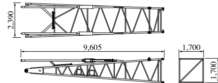
Tower Jib Top
